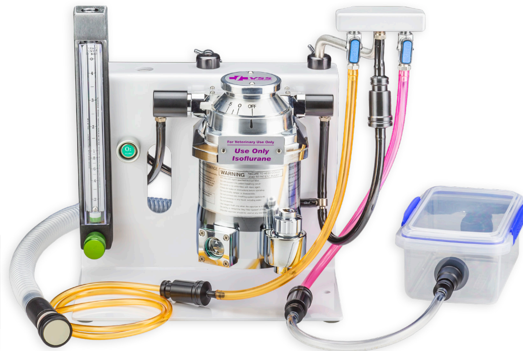
Optional Universal Control Arm Manifold for Bain Circuits P/N NA2013
